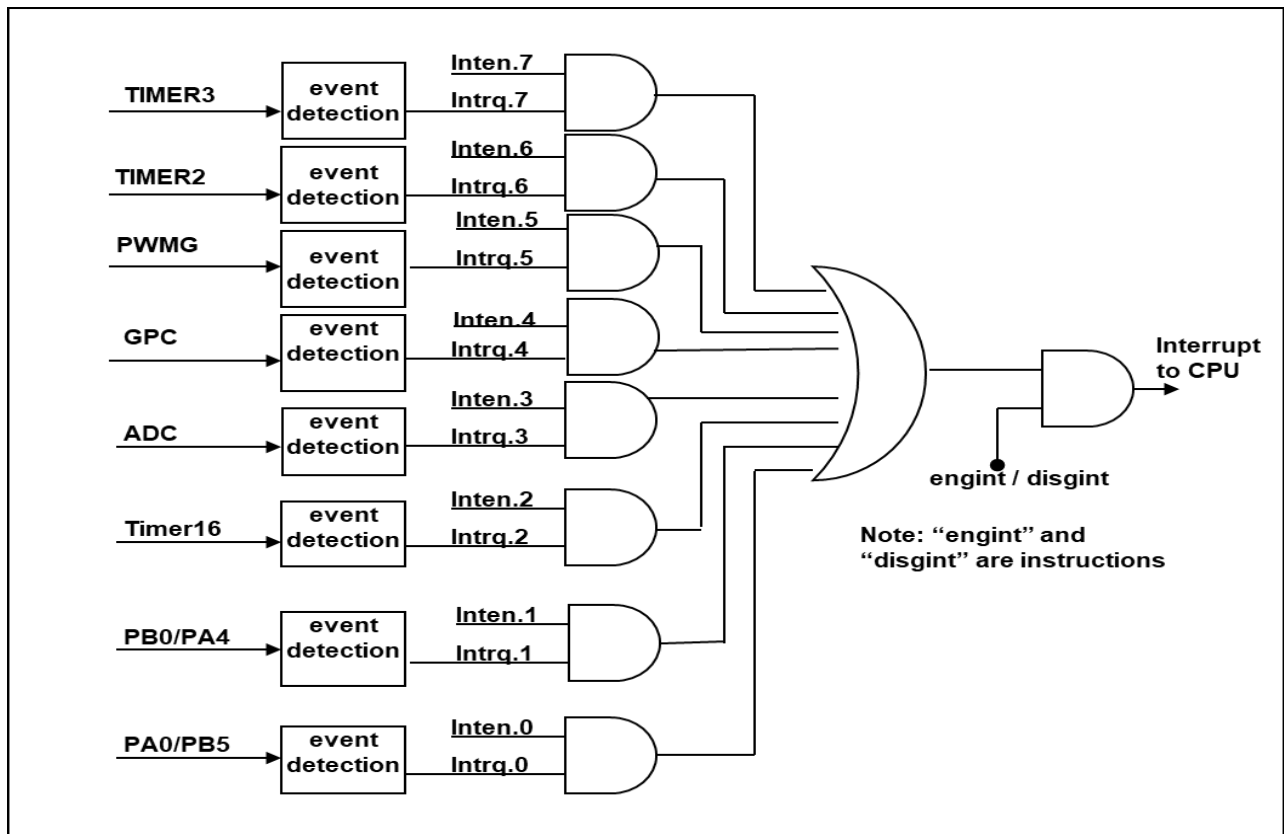
Fig.20: Hardware diagram of interrupt controller
