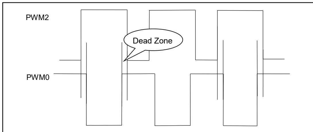
Fig.17: Complementary PWM waveform with dead zones
