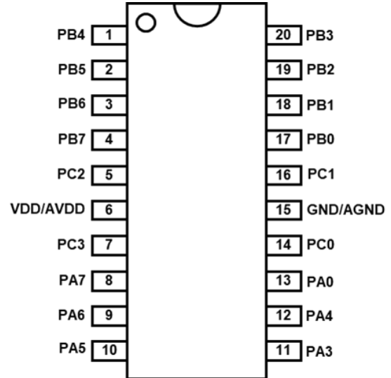
MF323-H20A (HTSOP20-150mil)
