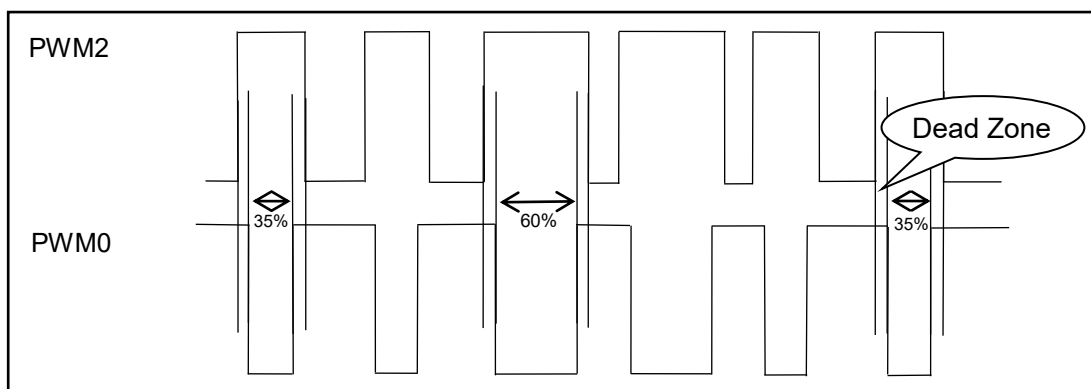
Fig.18: Complementary PWM waveform with dead zones
